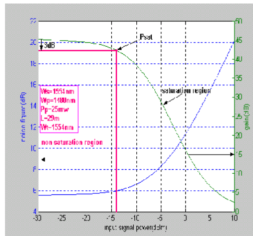
Fig.(24) NF and gain sat. vs. I/p power ( \lambda_p = 1480nm )
