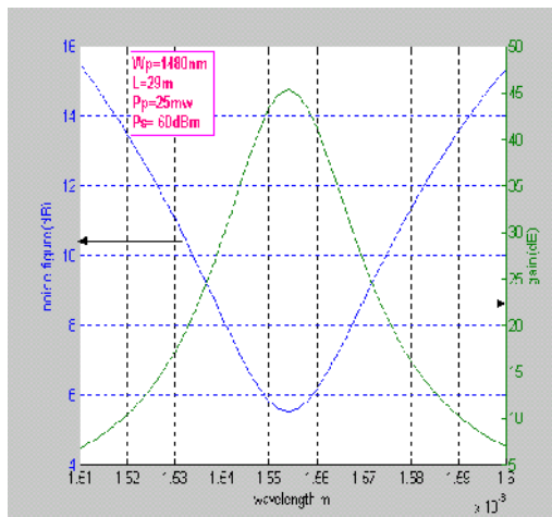
Fig.(22) NF and amp. gain vs. tran. wavelength
