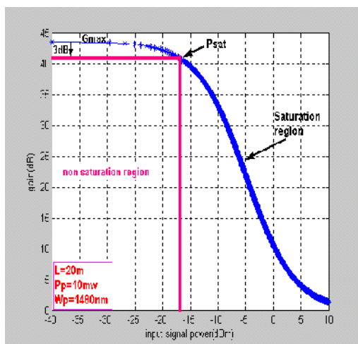
Fig.(10) amp. gain vs. input signal power ( \lambda_p = 1480\text{nm} )
