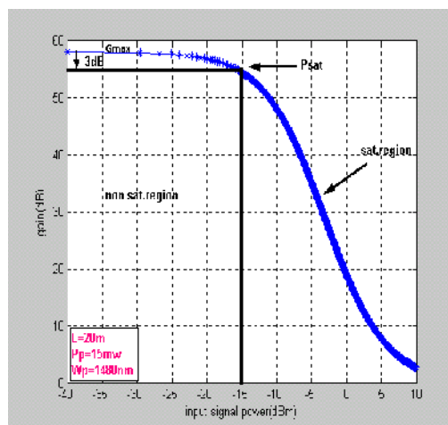
Fig.(11) amp. gain vs. input signal power ( \lambda_p = 1480\text{nm} )
