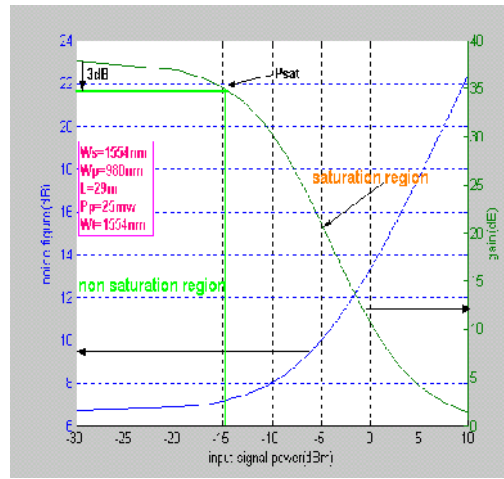
Fig.(25) NF and gain sat. vs. l/p power ( \lambda_p = 980nm )
